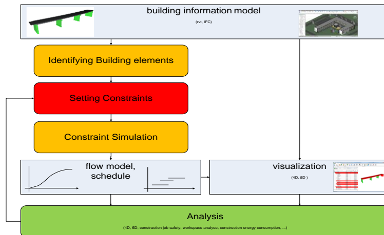
Figure 14: Constraint schedule simulation based on a Building Information Model
