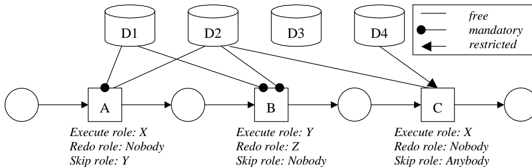
Figure 1: an example illustrating some of the case-handling concepts
