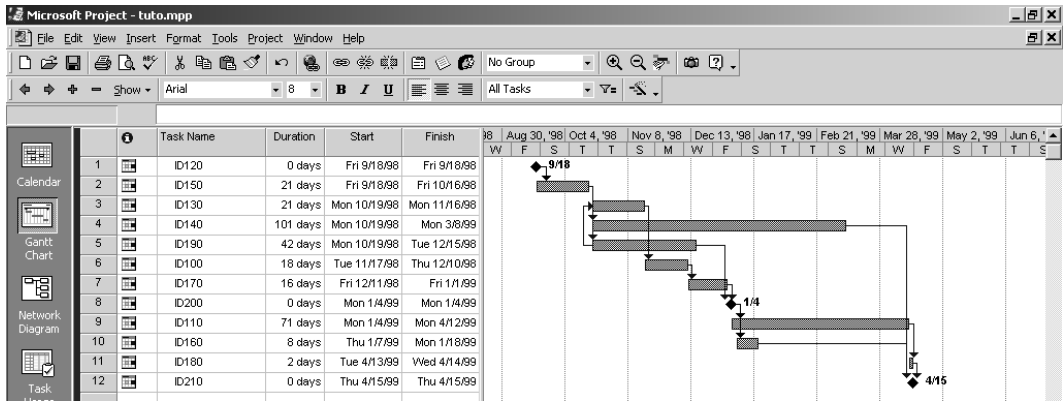
Figure 15. Regenerated Schedule in Microsoft Project using PSL
