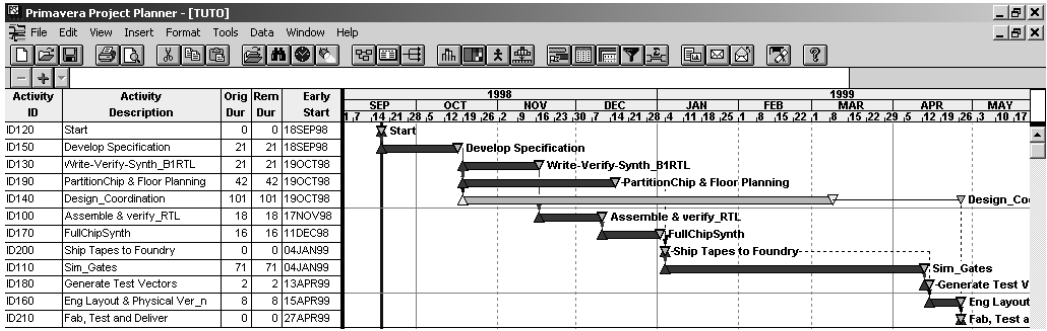
Figure 22. Group 1's Schedule in Primavera P3
