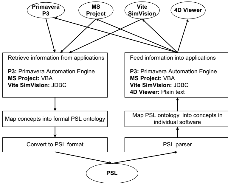
Figure 7. PSL Wrappers
